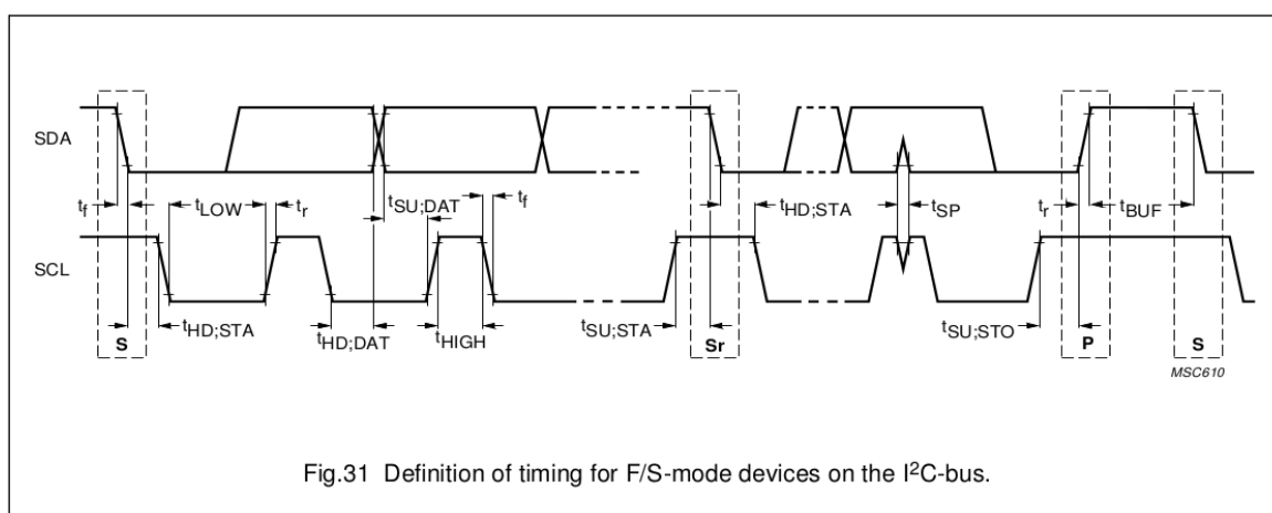
图 27.3-3. I2C 协议时序 (引自 The I2C-bus specification Version 2.1 Fig.31)
